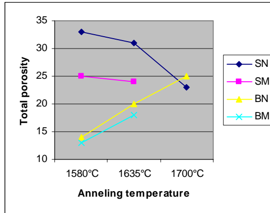
Fig. 2. Total porosity versus temperature
